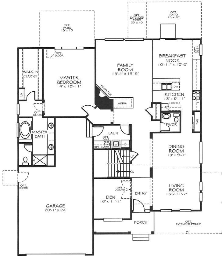
MAIN LEVEL
